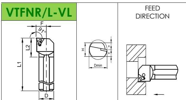
THE DRAWINGS RAPPRESENT RIGHT TOOLS • ANGLE OF INCLINATION = \Omega^\circ • SUPERIOR RELIEF ANGLE = -6^\circ
