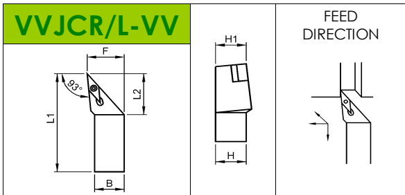
THE DRAWINGS RAPPRESENT RIGHT TOOLS • ANGLE OF INCLINATION = -0° • SUPERIOR RELIEF ANGLE = -0°
