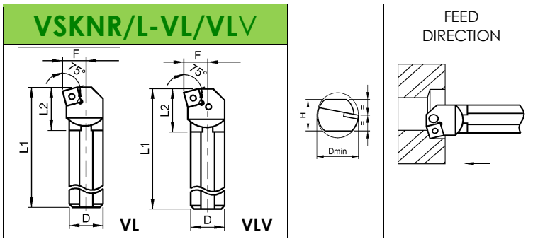
THE DRAWINGS RAPPRESENT RIGHT TOOLS • ANGLE OF INCLINATION = \Omega^\circ • SUPERIOR RELIEF ANGLE = -6^\circ
