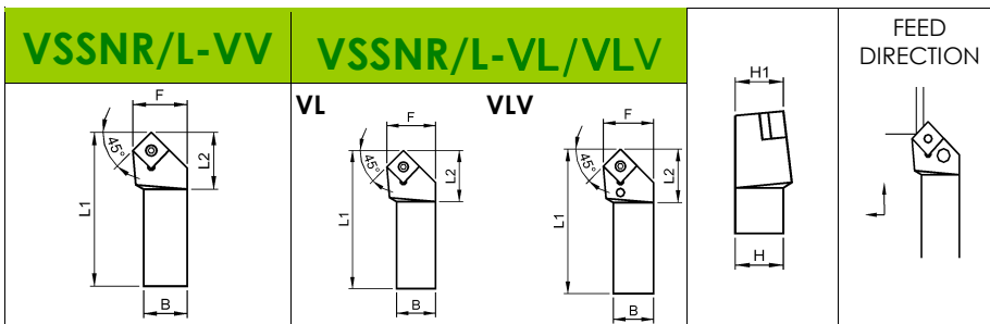
THE DRAWINGS RAPPRESENT RIGHT TOOLS • ANGLE OF INCLINATION = -0° • SUPERIOR RELIEF ANGLE = -8°
