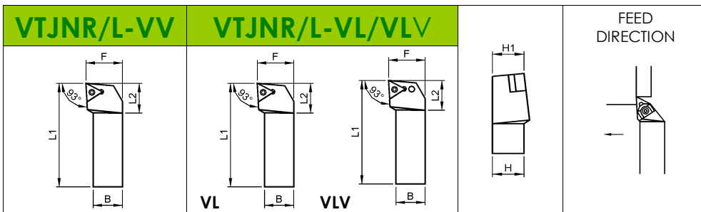
THE DRAWINGS RAPPRESENT RIGHT TOOLS • ANGLE OF INCLINATION = -6° • SUPERIOR RELIEF ANGLE = -6°
